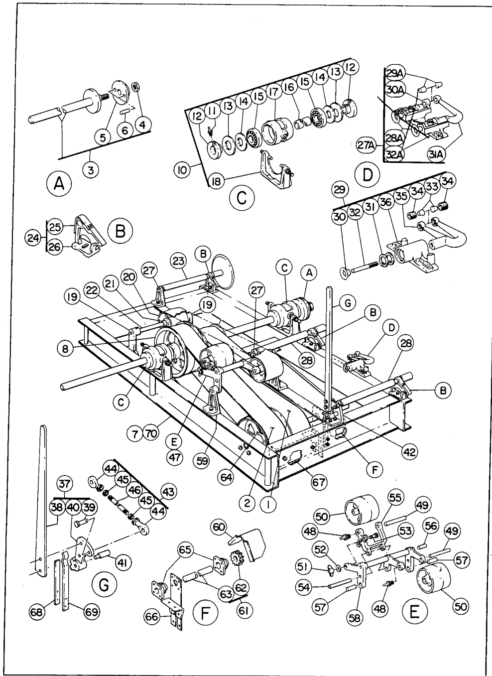
FIGURE 2 - HUSK ASSEMBLY
